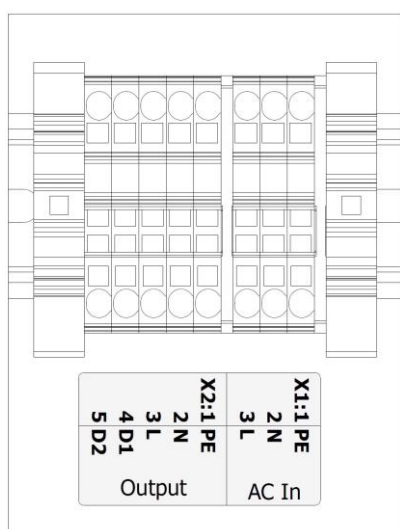
3. Electrical interface
