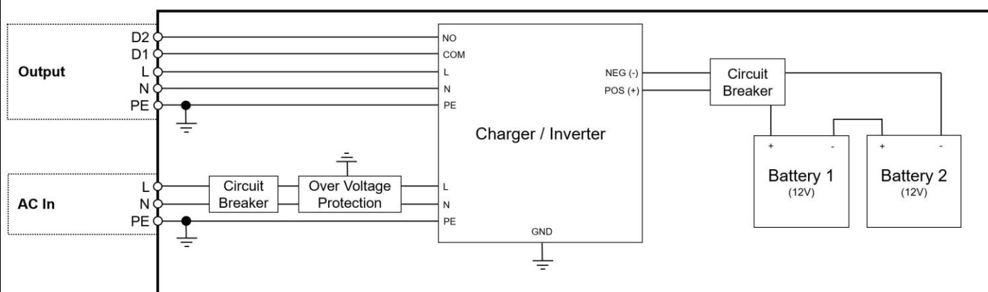
2. Block Diagram
