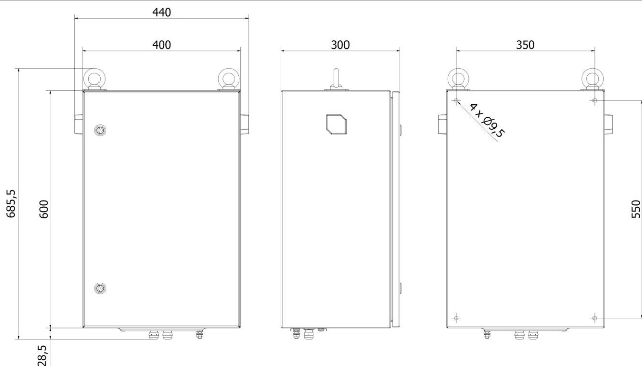
1. Cabinet dimensions
